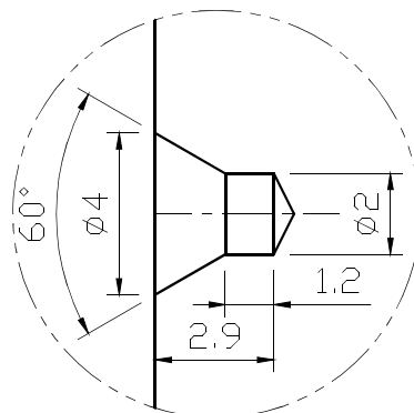
A section (10:1)
